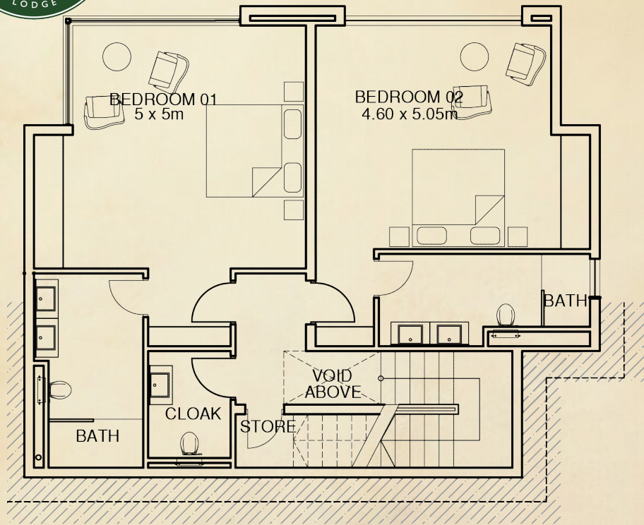
LOWER GROUND FLOOR 105 Sqm
